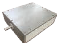
LBL600 Stroke [mm]: 35 Force [N]: 1000
