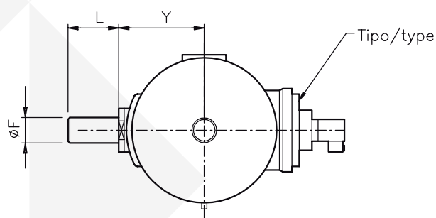
Valve blowpipe
